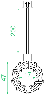
磁环 -75 A
